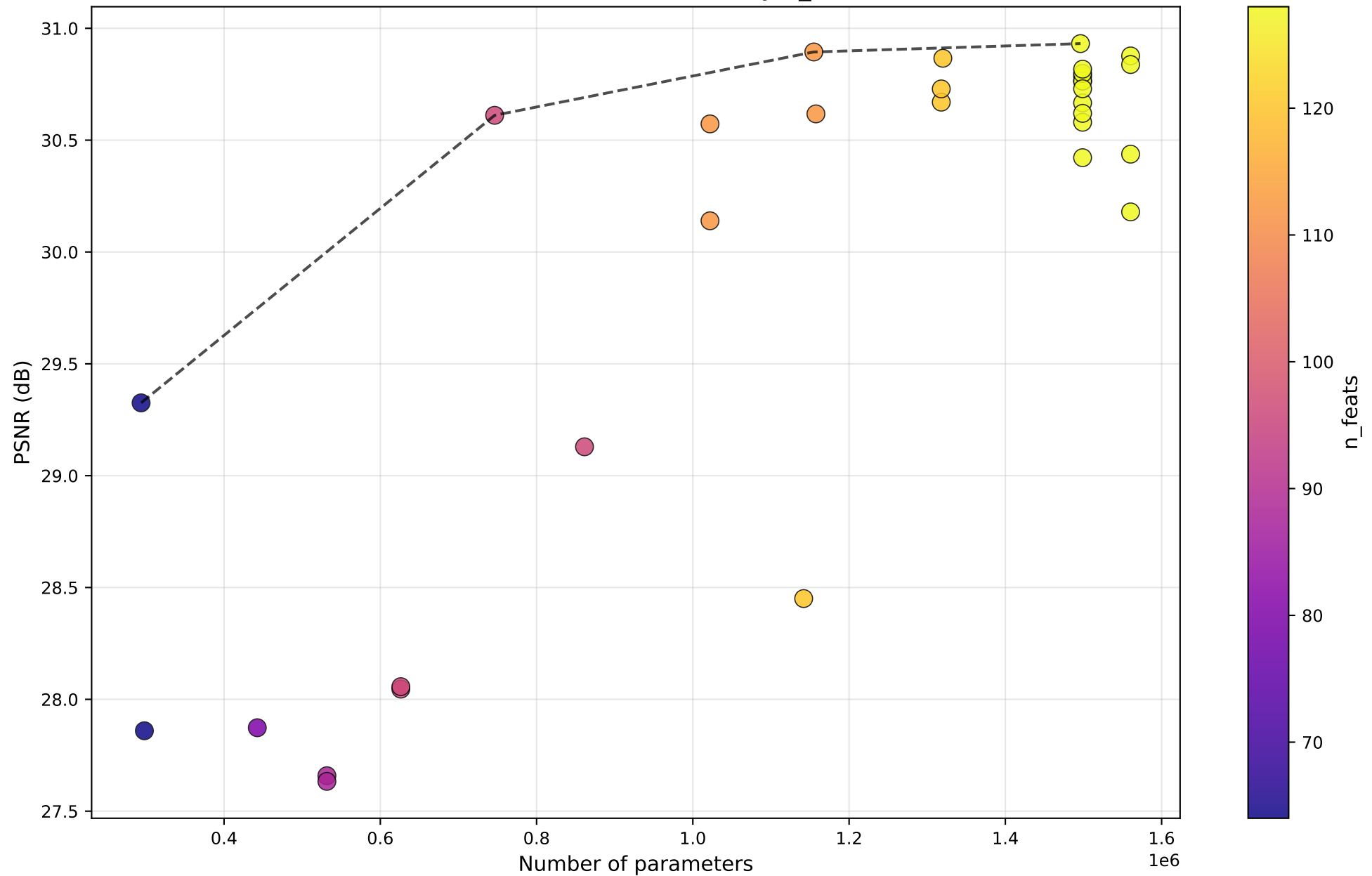
PSNR vs #Params — DAT — by n_feats
